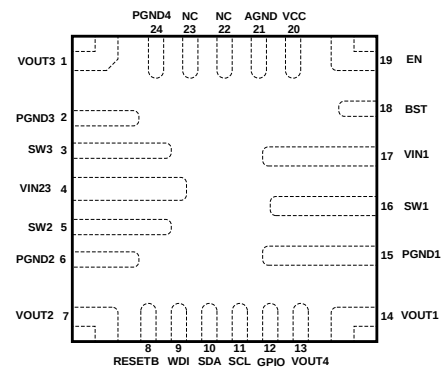
Top View: 24-Lead FCQFN 4mmx4mm
