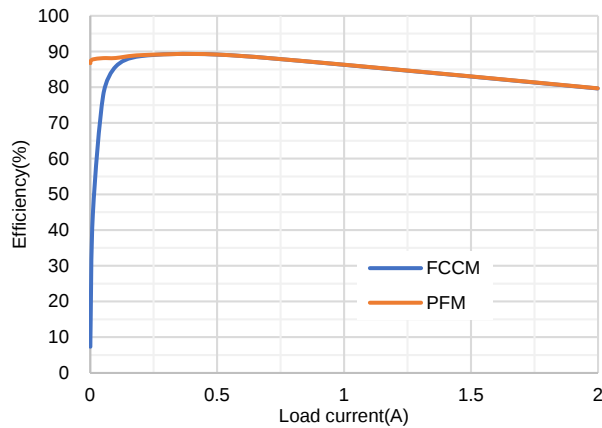
Buck2/3 Efficiency vs Load Current, V_{OUT2/3}=1.2V
