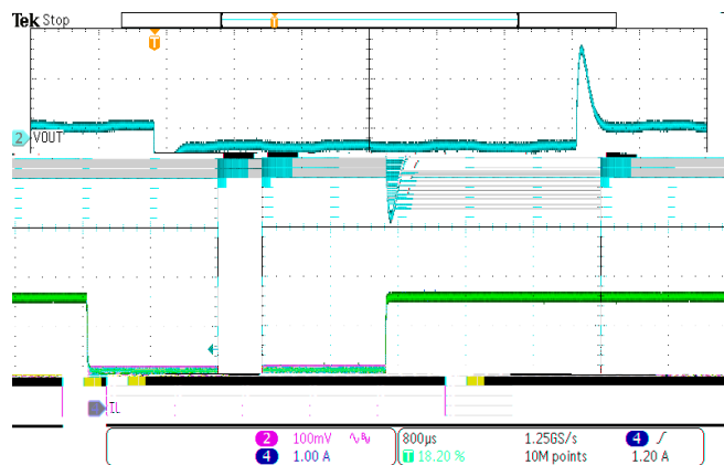
Figure 21. Load Transient VOUT=5V, IOUT=0.75A to 2.25 A, SR=250mA/us
